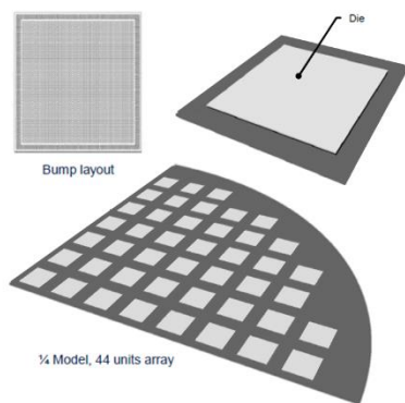
Fig. 12. Mold flow simulation model.
