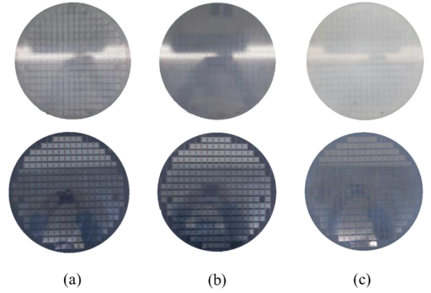
Fig. 6. Molded wafer and ground wafer of: (a) EMC-1, (b) EMC-2 and (c) EMC-3.
