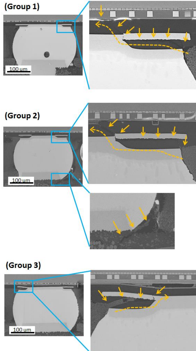
Figure 6. Cross-sectional images of drop test failures.
