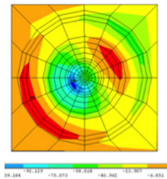
Low-k stress
